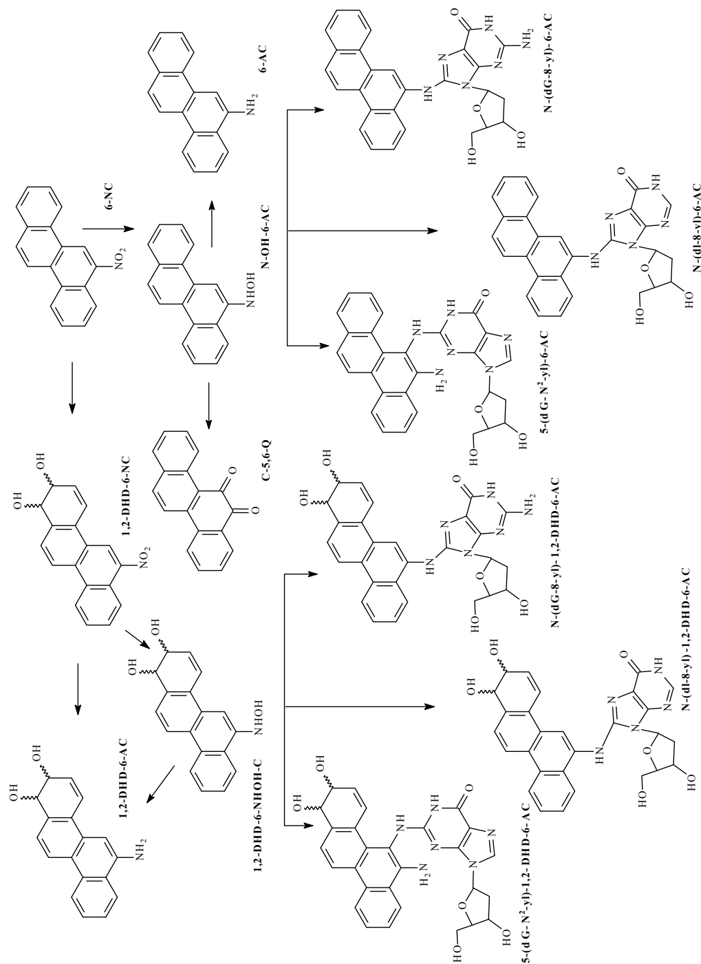
Fig. 4.1 Metabolism and DNA-adduct formation of 6-nitrochrysene
